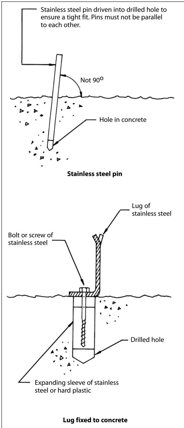
Figure 2: Mechanical fixing devices
