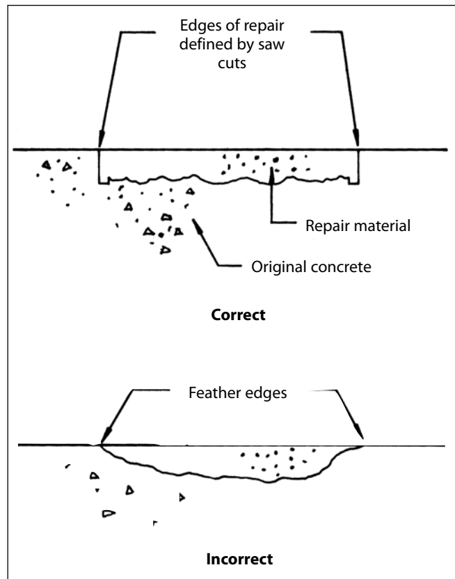
Figure 1: Edges to repairs – use saw cuts to avoid feather edges
