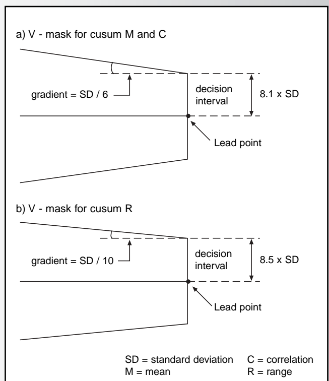
Figure 5: v-mask design for concrete cusum (modified from reference 1)
